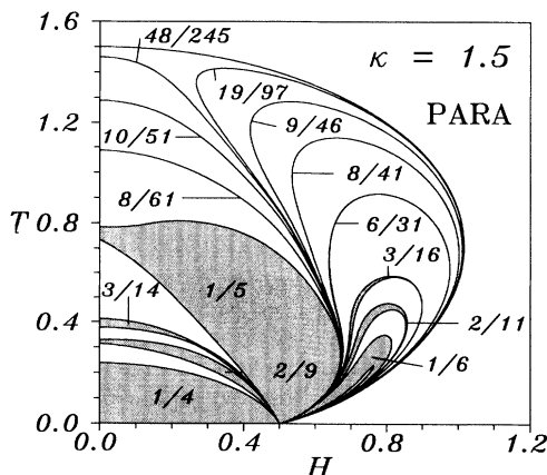
FIG. 13. T - H phase diagram for \kappa = 1.5 .
