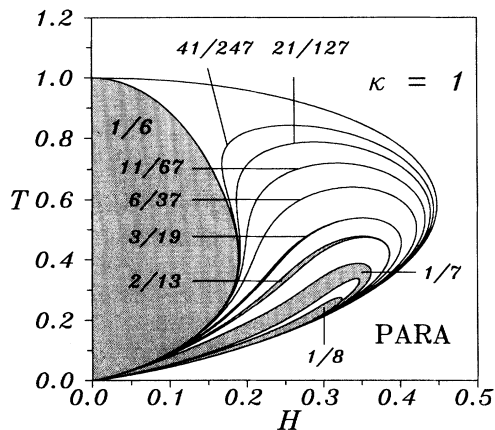
FIG. 10. T - H phase diagram for \kappa = 1 .
