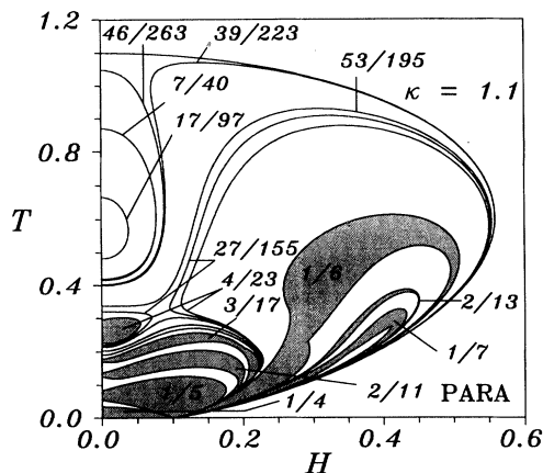
FIG. 12. T - H phase diagram for \kappa = 1.1 .
